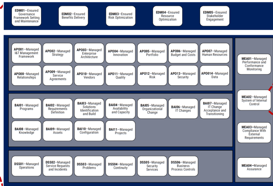
Figure 4.2 COBIT Core Model
